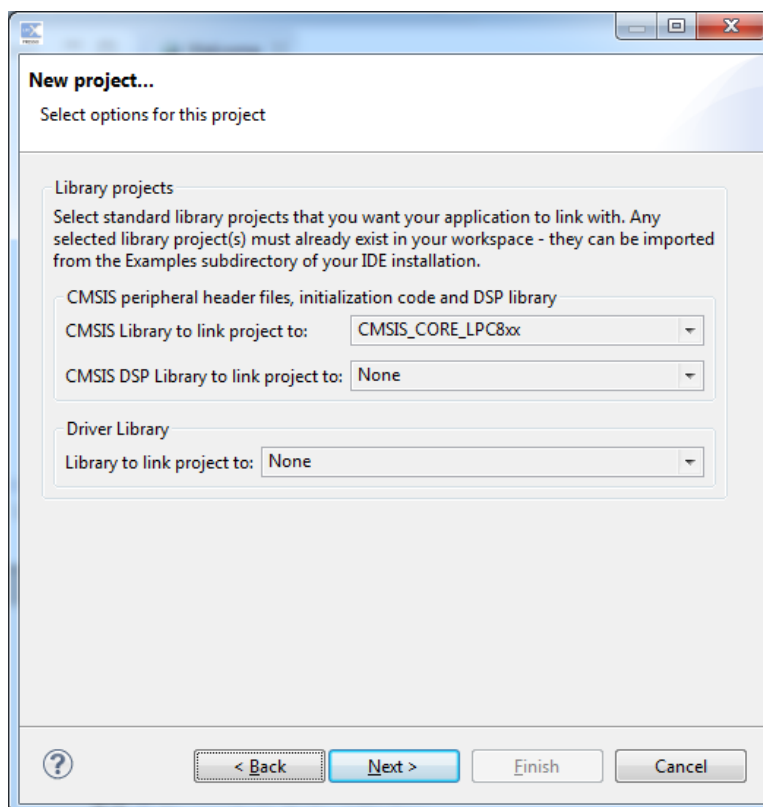
Fig 32. CMSIS selection
