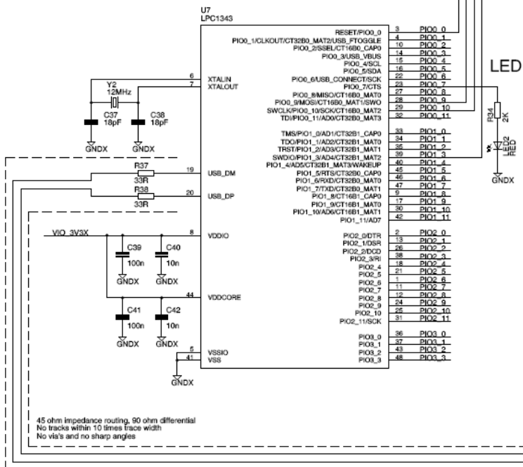
Fig 38. Schematic for the LPCXpresso LPC1343 target side 2
