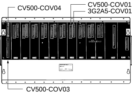
CPU Rack
