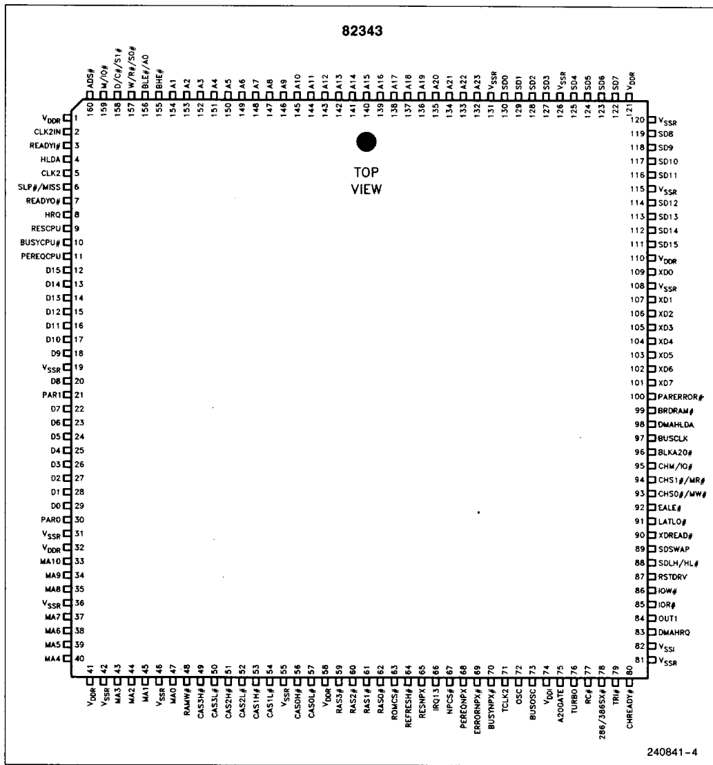
Pin Diagram
