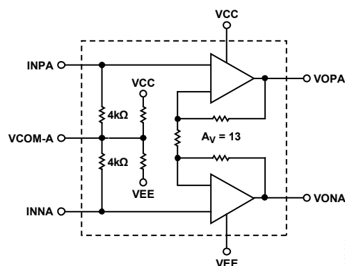
Figure 2. Channel A Internal Schematics
