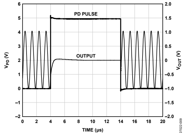
Figure 9. Power-Down/Power-Up Transition
