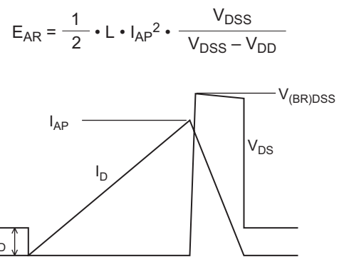
Avalanche Waveform
