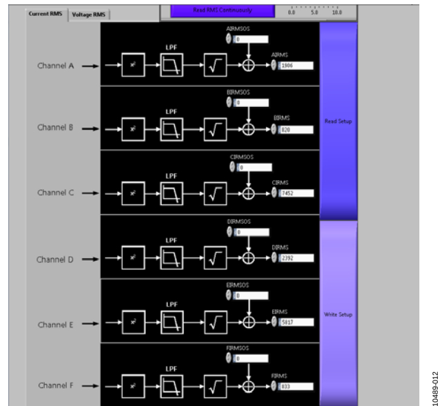
Figure 12. RMS Window
