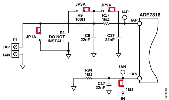
Figure 4. Typical Current Channel A Configuration with a Rogowski Coil
