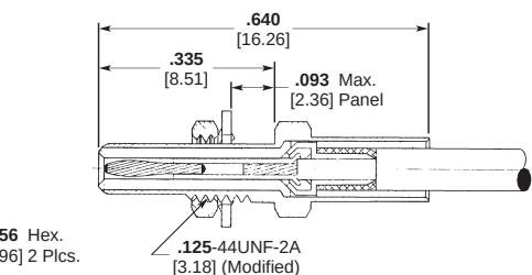
Straight Bulkhead Jack 1 Part Number 141-1001-0001 Instruction Sheet Number 408-08512 Former MICRODOT I.S. Number RF-ASMB-15
