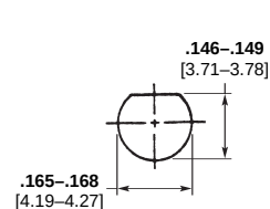
"D" Hole Dimensions For Panel Mounting
