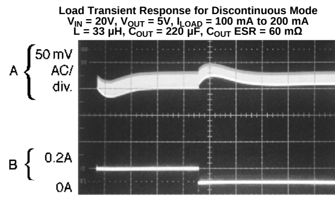
Figure 17. Horizontal Time Base: 2 \mu\text{s}/\text{div} .
