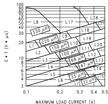
Figure 24. LM2594/LM2594HV-ADJ
