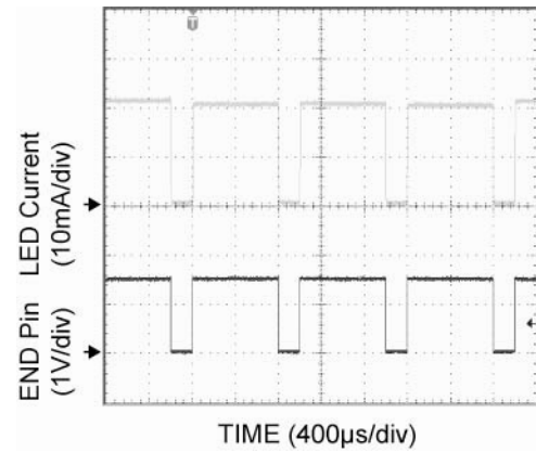
Figure 9. PWM Signal at 80% Duty Cycle ( I_{avg} = 16mA )
