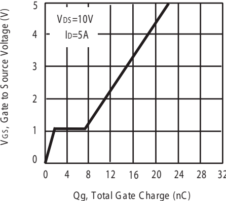
Figure 9. Gate Charge
