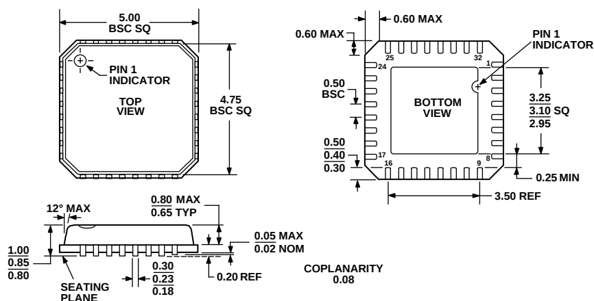
Figure 42. 32-Lead Lead Frame Chip Scale Package [LFCSP] 5 mm × 5 mm Body (CP-32-2)
