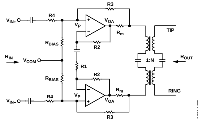
Figure 37. Typical ADSL/ADSL2+ Application Circuit
