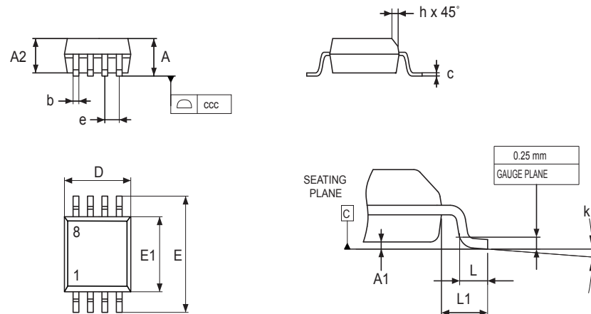
Figure 28. SO8N – Outline
