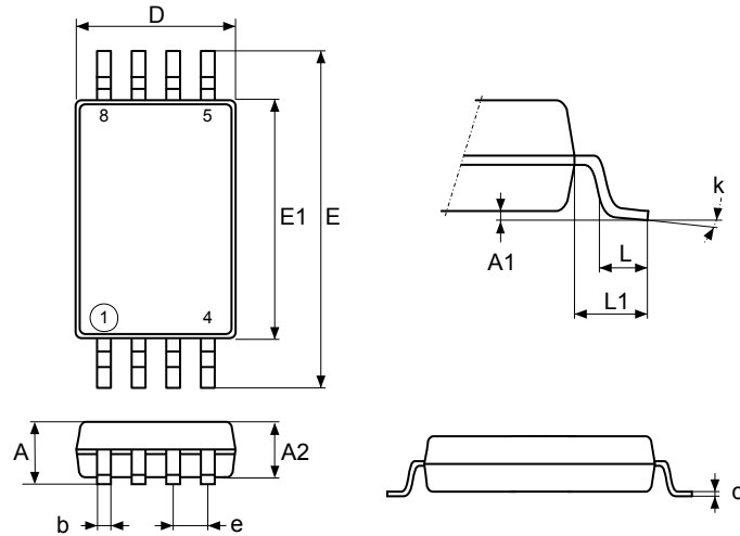
Figure 26. TSSOP8 – Outline
