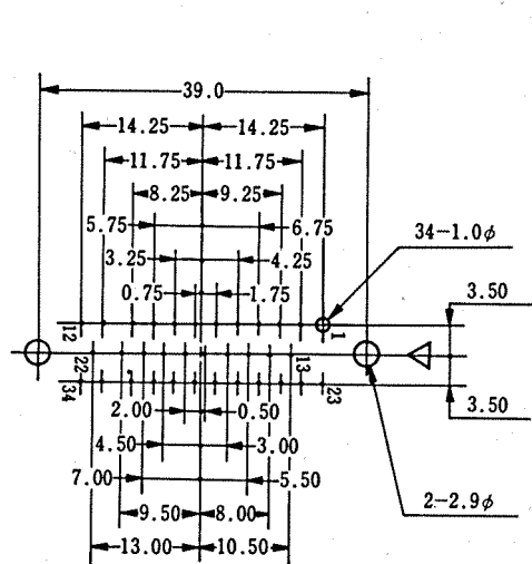
SD-1634
