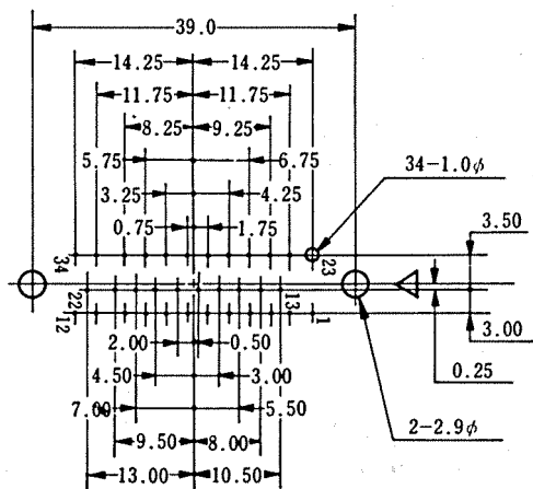
PD-1634
