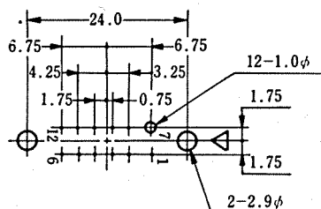
PD-1612
