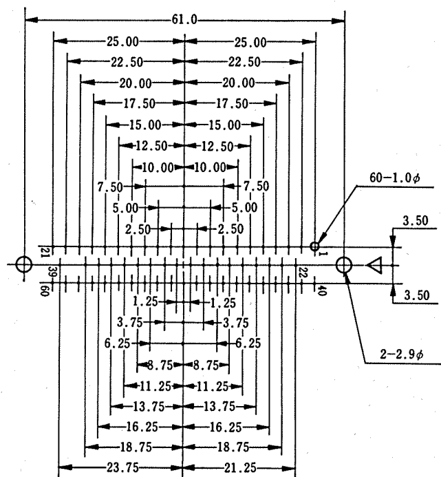
SD-1660
