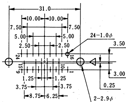
PD-1624
