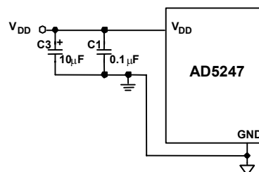
Figure 11. Power Supply Bypassing
