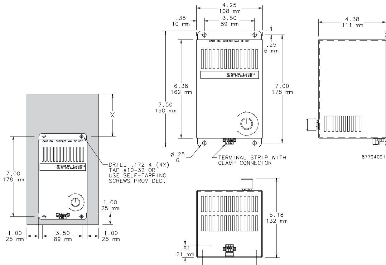
Dimensions and Clearance Range Drawing for DAH4001B, -2B and DAH8001B, -2B
