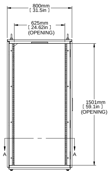
L.S. VIEW
