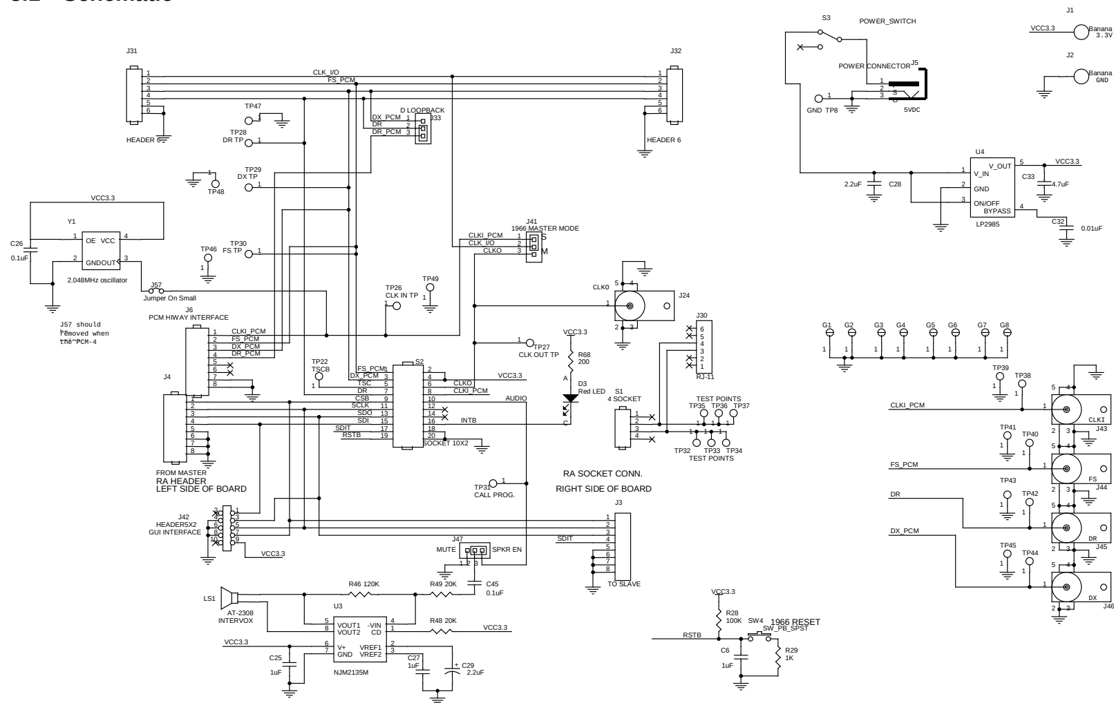
Figure 5: 73M1966 Motherboard Schematics
