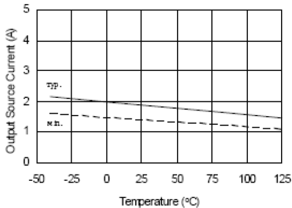
Figure 14A. Output Source Current vs Temperature
