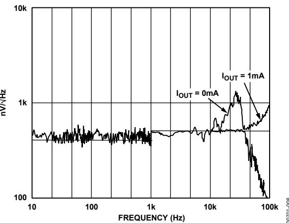
Figure 8. Noise Spectral Density
