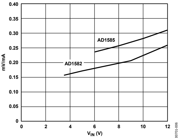
Figure 6. Load Regulation vs. V_{IN}
