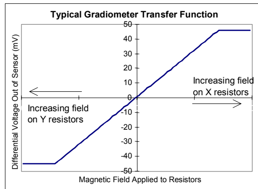
GRADIOMETER BRIDGE SENSOR OUTPUT CHARACTERISTIC
