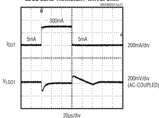
LD02 LOAD TRANSIENT WAVEFORM
