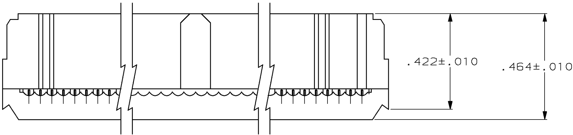
TERMINATED VIEW
