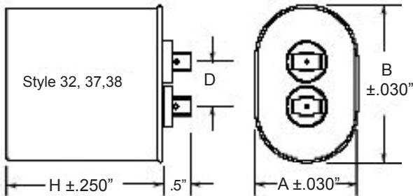
Oval Case Style
