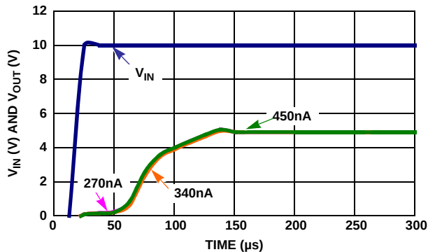
FIGURE 53. TURN-ON TIME
