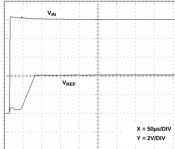
FIGURE 39. TURN-ON TIME
