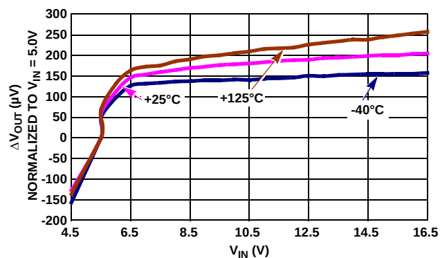
FIGURE 33. LINE REGULATION OVER-TEMPERATURE
