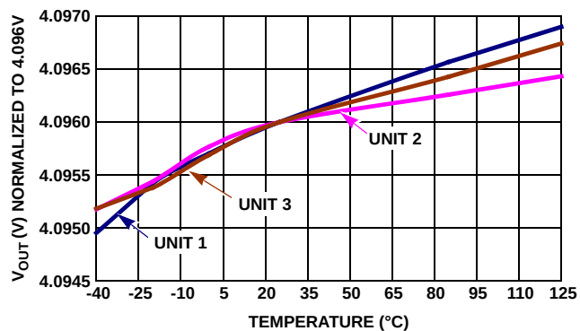
FIGURE 35. V_{OUT} vs TEMPERATURE
