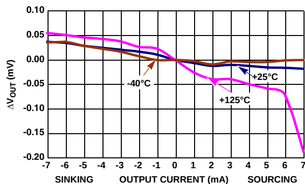
FIGURE 34. LOAD REGULATION
