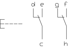
10 Pushbutton actuator two-part page 7 | Pushbutton actuator locked mechanically page 8
