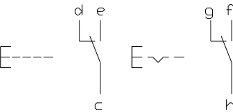
12 Pushbutton actuator two-part page 7
