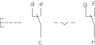
7 Pushbutton actuator one-part page 6
