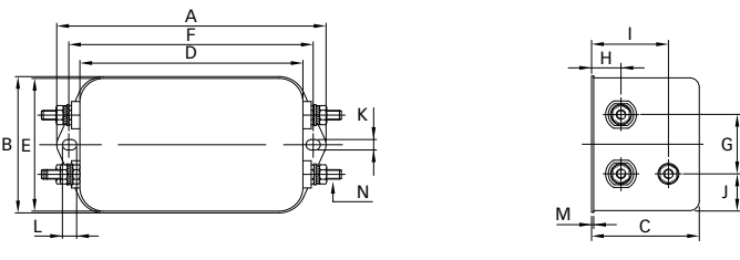
Connection style -08, 20A types
