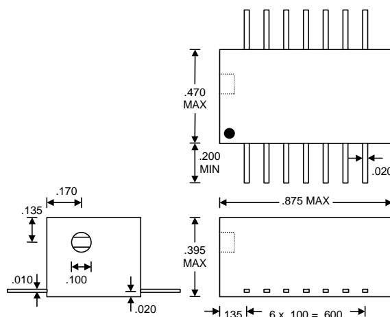
Package Dimensions
