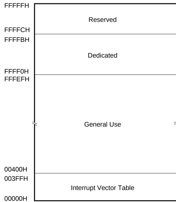
Figure 2-2. Interface with Memory (1/2)
