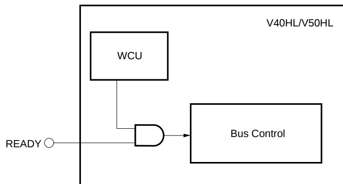
Figure 7-3. WCU and READY Control
