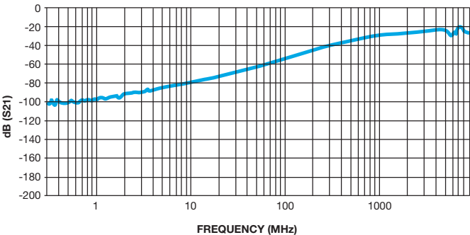
Typical AVX W2F43A1018AT Typical Far-side XTALK Elements 1 - 3
