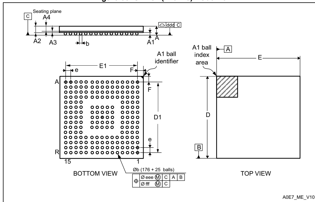
Figure 88. UFBGA(176+25) - Outline
