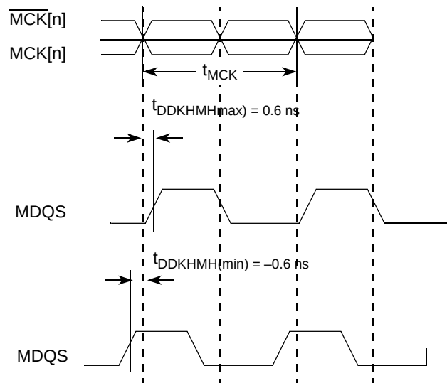
Figure 5. Timing Diagram for t_{DDKMH}
