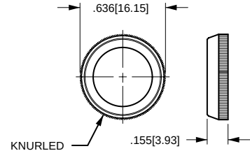
"DRESS" FACENUT .636" X .155" [16.15] X [3.93] NICKEL - 380-08810 BLACK - 380-08811
