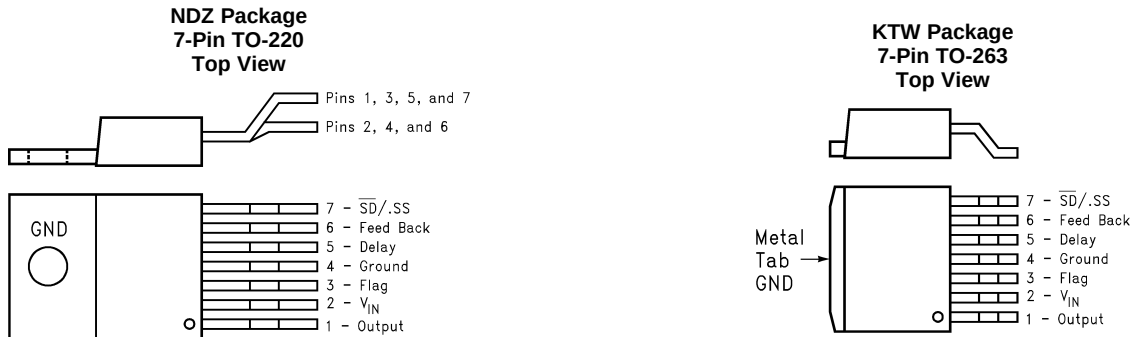
Pin Functions
