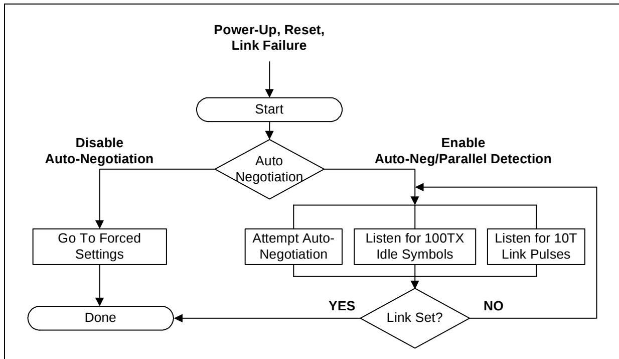
Figure 12. Auto-Negotiation Operation
