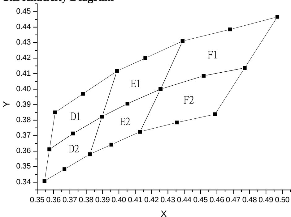
Color Ranks (IF=20mA , Ta=25°C)
