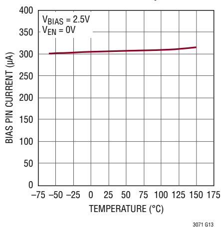
BIAS Pin Current in Nap Mode
