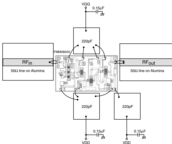
ASSEMBLY DRAWING
