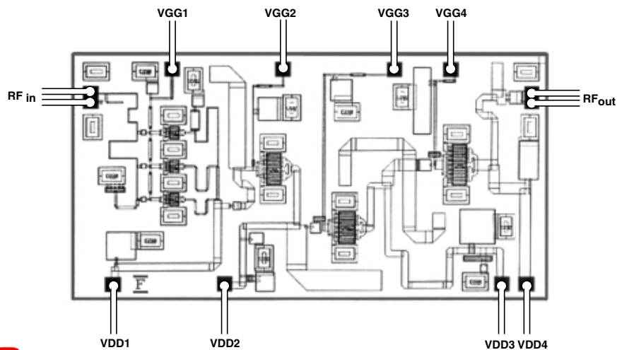
BONDING LAYOUT
