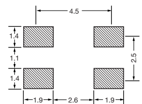
Figure 5) ECX-64CEN - Recommended Solder Pad Layout
