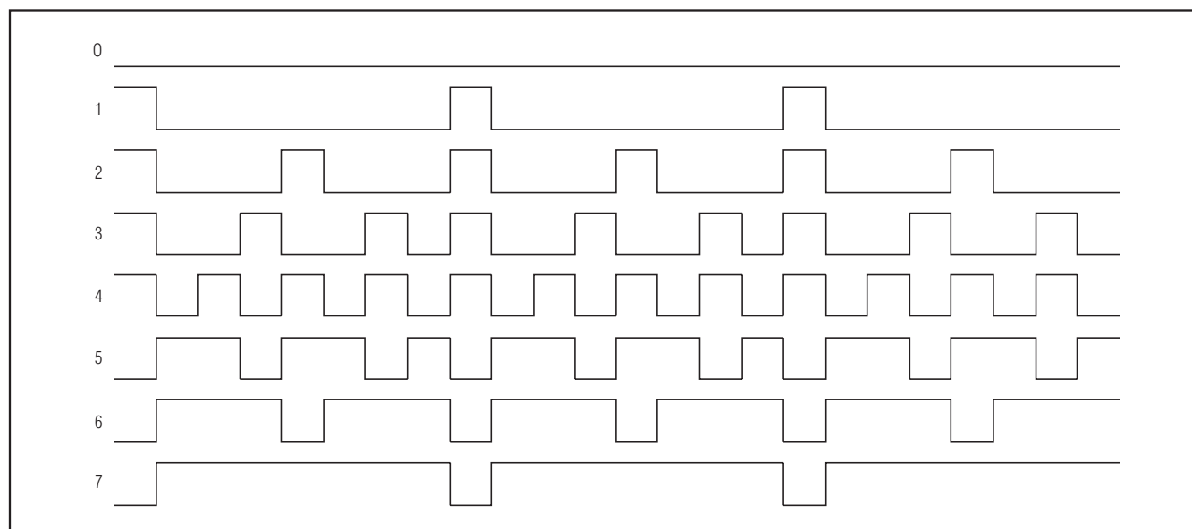
Figure 12. Delta-Sigma Outputs
