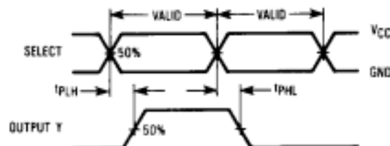
Figure 2. Switching Waveforms
