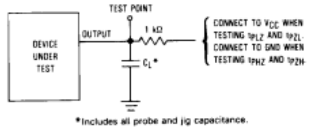
Figure 5. Test Circuit
