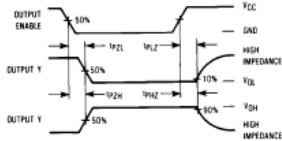
Figure 3. Switching Waveforms
