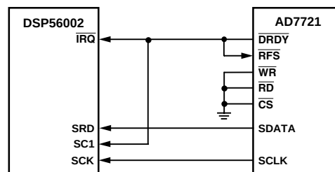
Figure 14. AD7721 to DSP56002 Interface
