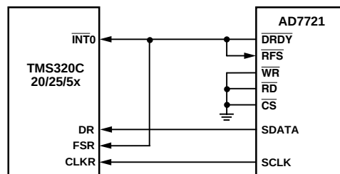
Figure 15. AD7721 to TMS320C20/25/5x Interface
