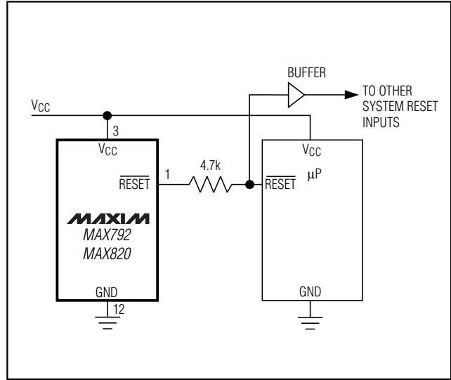
Figure 12. Interfacing to \mu\text{Ps} with Bidirectional RESET Pins
