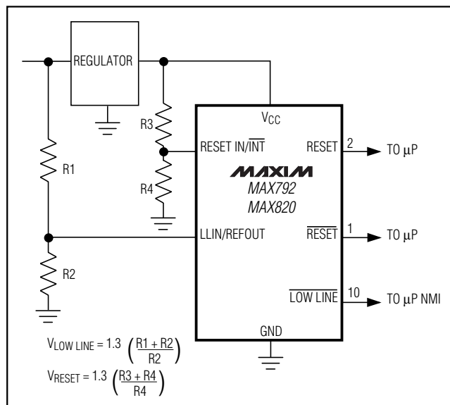
Figure 4c. Alternative Connection for External Programming Mode
