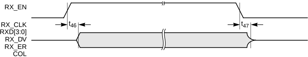
Figure 6.8 RX_EN Timing
