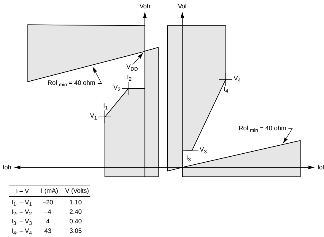
Figure A.4 MII Output Driver Characteristics
