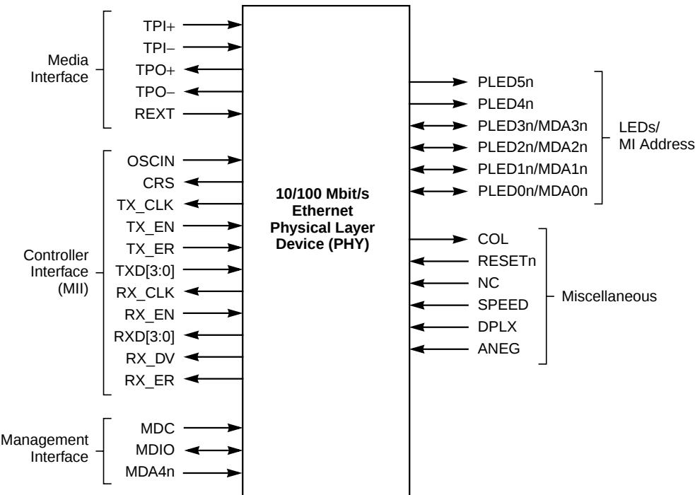
Figure 3.1 Device Logic Diagram
