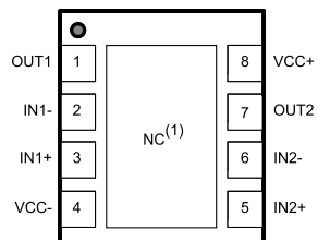
DFN8 2x2
