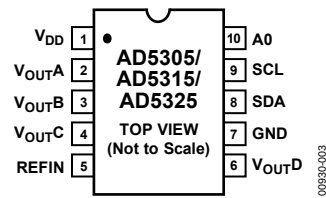
Figure 3. Pin Configuration
