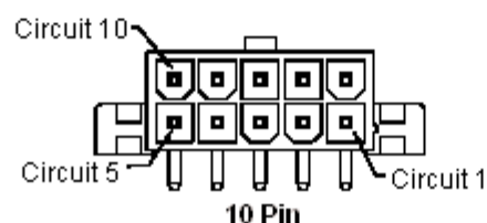
2 to 20P Protection Key Drawing
