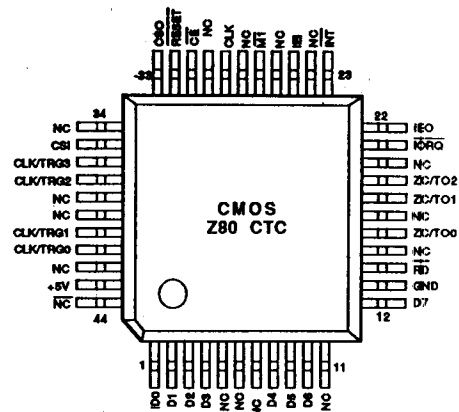
Figure 2C. 44-Pin LOFP Pin Assignments
