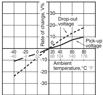
5-2. Ambient temperature characteristics (1 Form A 1 Form B)
