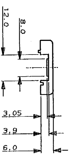
VIEW "A"
