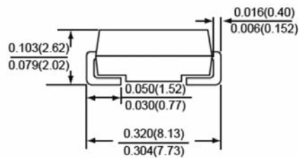
SMC/DO-214AB
