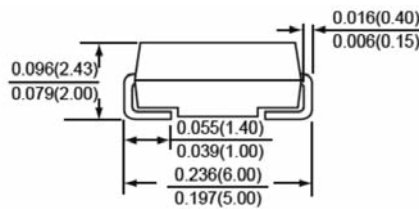
SMB/DO-214AA
